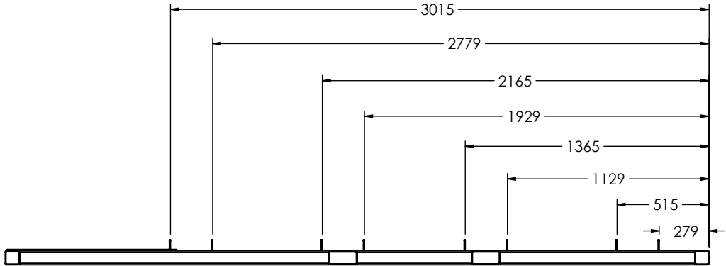
RIGHT VIEW
