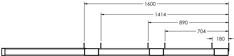
RIGHT VIEW
