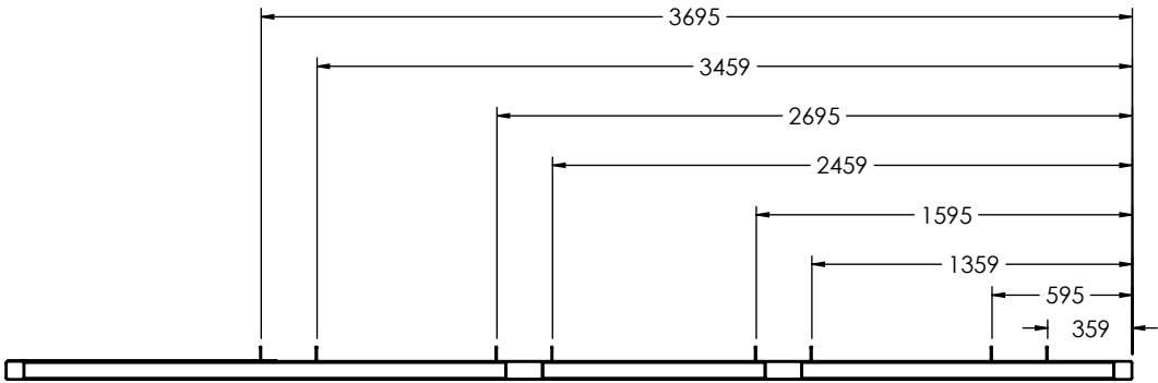
RIGHT VIEW
