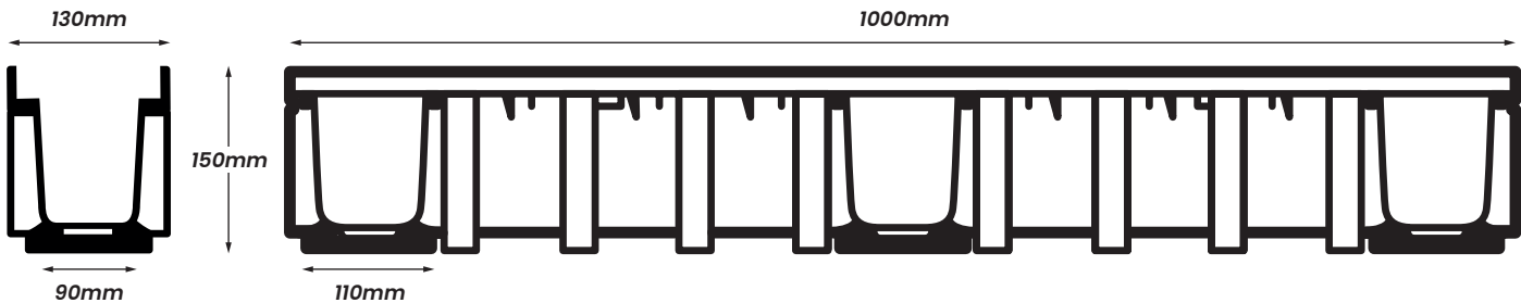
150mm Depth
