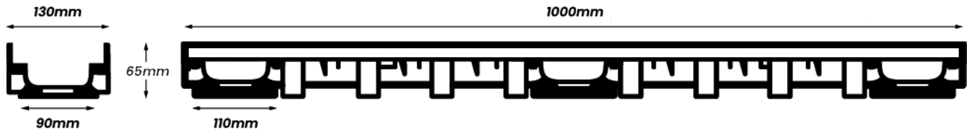
100mm Depth
