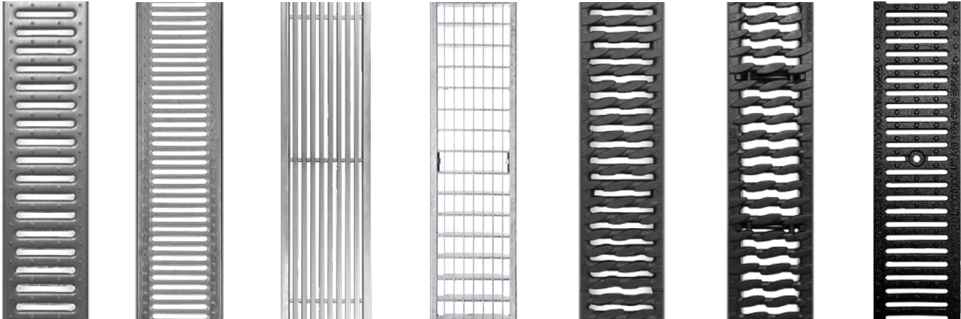
Galvanised Slotted Grating (A15) Galvanised SafeHeel Slotted Grating (A15) Longitudinal Steel Grating (A15) Mesh Steel Grating (B125) Plastic OvalGrip Grating (B125) Ductile Iron OvalGrip Grating (B125) KTL Frosted Ductile Iron Slotted (B125)
